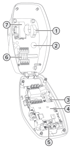
Fig. 3: Interior view
