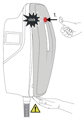
Fig. 20: Anbring front cover - 1
