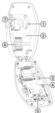
Fig. 3: Vista interior
