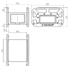
Drawing 5 MB 76 Dim. in mm
